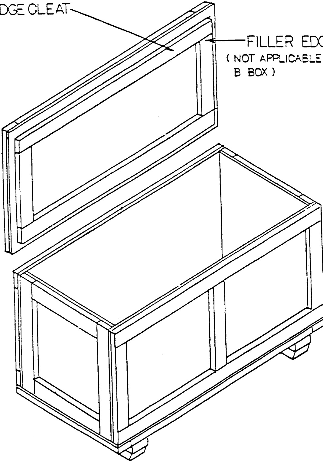
TOP PANEL MODIFICATION OF UNNAILED CLOSURE, STYLE A, BOX FIGURE 1-A
